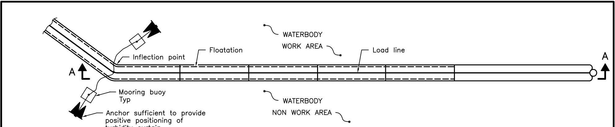
PLAN
