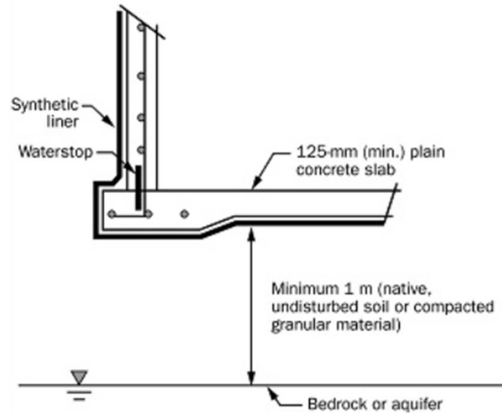
Diagram 4 — Lined, unreinforced floor
